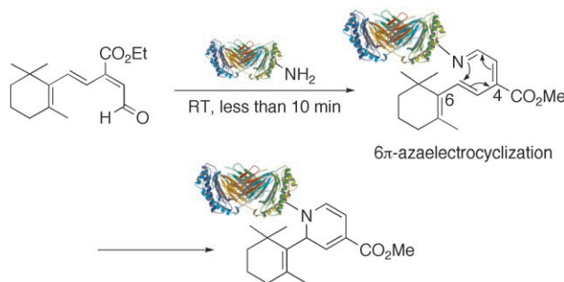
Scheme 1. Rapid reaction with lysine through 6 \pi -azaelectrocyclization.
